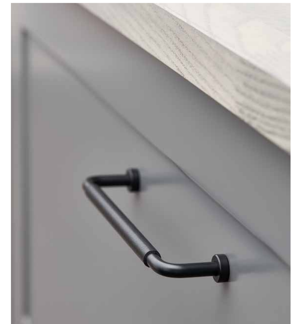
LOUNGE 240330160 Design furnipart Material Stainless steel Finish 102/9005 - Black leather/Black Centre distance 160 Centre 174 Width - Height 35 Diameter 7/14
